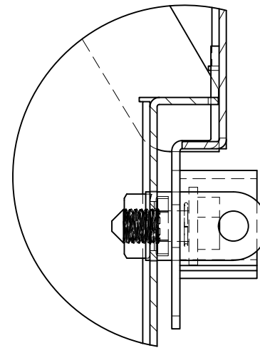
DETAIL L SCALE 1:2
